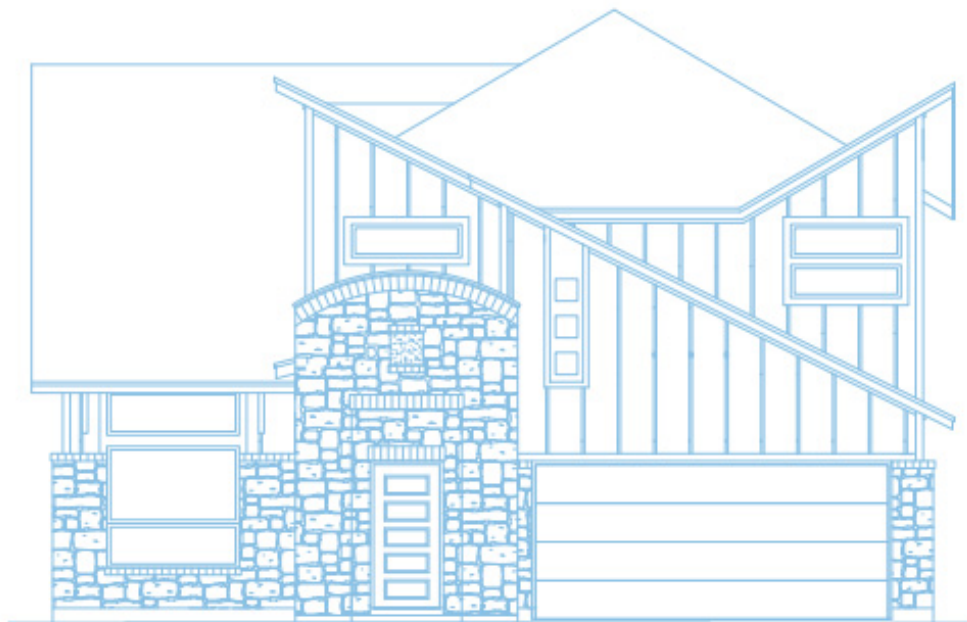
Elevation D
